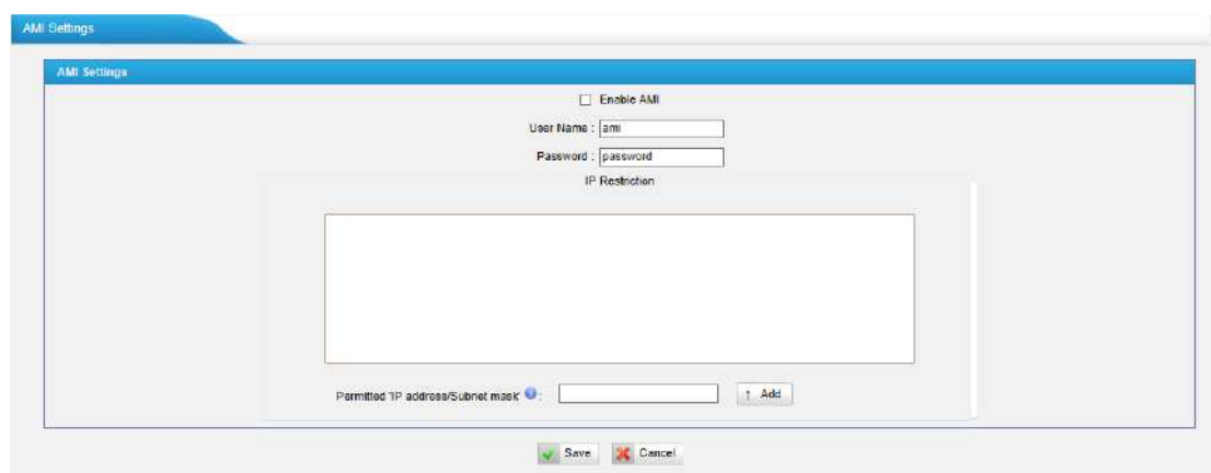
Figure 10-5 AMI Settings
