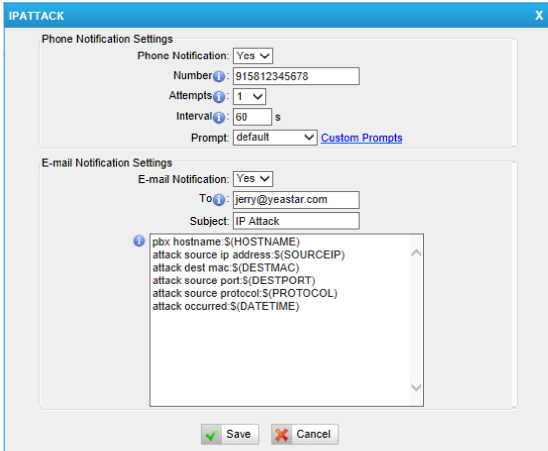
Figure 10-4 Alert Settings
