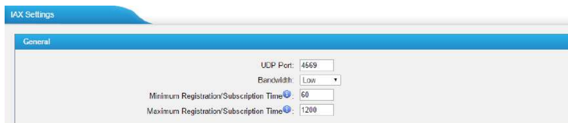
Figure 5-10 IAX Settings
