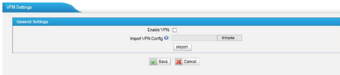
Figure 9-6 VPN Settings
