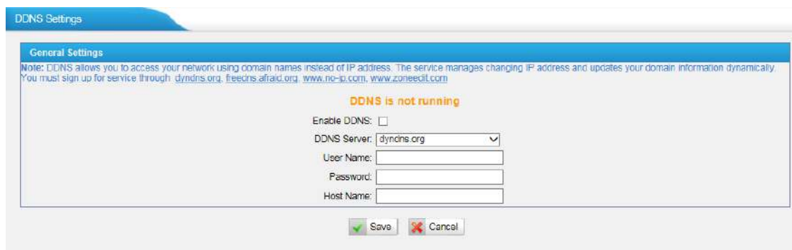
Figure 9-7 DDNS Settings
